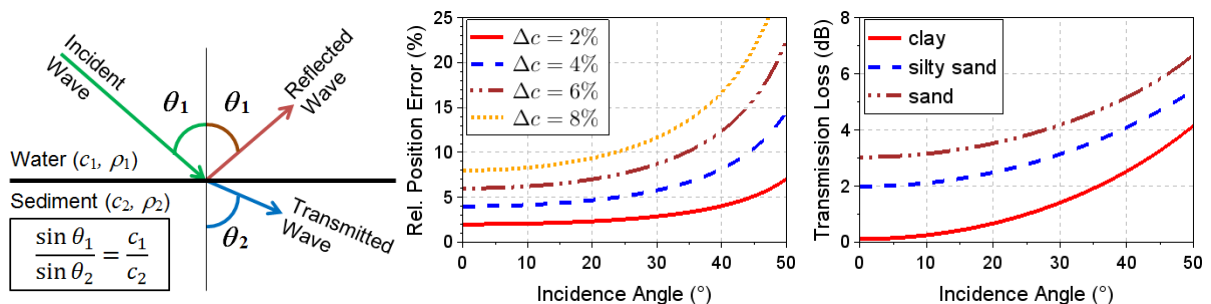
Figure 2: Sound wave reflection and refraction at a flat water-sediment interface with incidence angle \theta_1 , the same angle for the reflected wave front and angle \theta_2 of refracted wave front transferred into the seabed ( left ) Position error due to refraction (Euclidian distance between true and mapped cable position related to true burial depth) depending on incidence angle for sand at different sound speed estimation errors ( centre ). Two-way transmission loss TL [3] at a smooth water-seabed interface for different sediment types depending on incidence angle ( right ).
