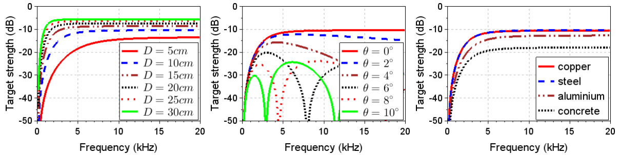
Figure 1: Target strength depending on frequency of a cable modelled as infinite steel cylinder buried in sand [4] for different diameters D at normal incidence ( left ), for different incidence angles \theta with diameter D = 10\text{cm} ( centre ) and for different cylinder materials at normal incidence ( right ).
