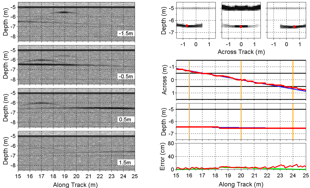
Figure 7: Four narrow-beam projectors and four hydrophones spread across-track 1m apart following a cable according to the model shown in Fig. 4: echo prints of the four hydrophones ( left ); estimated (red) and true (blue) cable positions across track and burial depth; burial depth error (green) and total position error as Euclidian distance (red); projector/receiver positions shown in black ( right ). Only the central ten metres of the model are shown. Cable position estimated from energy focusing. Much lower position errors than seen in Fig. 6.
