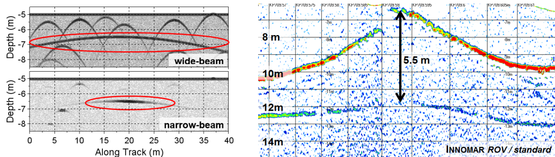
Figure 5: Model echo prints from a cable (red marks) buried 1.5m below seafloor surveyed along track according to the model shown in Figure 4 (3.5m off-track at start/end) and boulders spread in the seabed, for a linear wide-beam and a parametric narrow-beam system; boulders at the same locations for both data sets ( left ). Data example showing a pipeline followed along-track with burial depth up to 5+m; pipeline echo level is decreased with increasing burial depth due to increasing sound attenuation; echo level reduction might be partly caused by the survey vehicle coming off-track, thus exact pipe position cannot be obtained ( right ).
