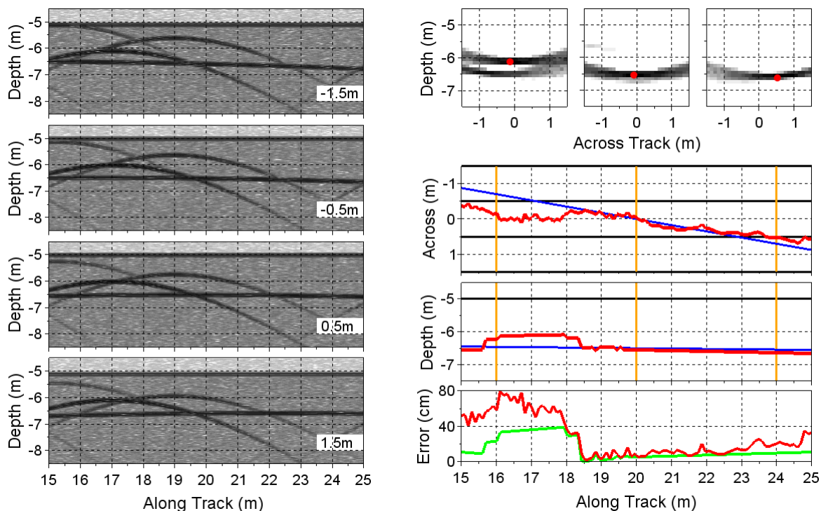
Figure 6: One wide-beam projector covering the full swath and four hydrophones spread across-track 1m apart following a cable according to the model shown in Figure 4: echo prints of the four hydrophones ( left ); estimated (red) and true (blue) cable positions across track and burial depth; burial depth error (green) and total position error as Euclidian distance (red); receiver positions shown in black ( right ). Only the central ten metres of the model are shown. Cable position estimated from energy focusing. Large position errors due to boulders and refraction.
