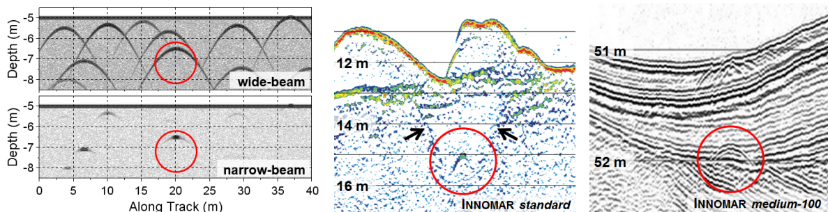
Figure 3: Model echo prints from a cable (red marks) buried 1.5m below seafloor surveyed across track and boulders spread in the seabed, for a linear wide-beam and a parametric narrow-beam system; boulders at the same locations for both data sets ( left ). Data example showing a pipeline approx. 4m below sand, trench is visible (arrows), original seabed below sand waves ( centre ). Data example showing a 12cm-cable buried about 1m below seafloor at 51m water depth surveyed shortly after dredging, diffraction hyperbolas visible at the seabed due to remaining trench banks ( right ).
