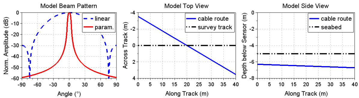
Figure 4: Model used: linear (blue) and parametric (red) beam patterns, half-power beam width linear 50° and parametric 5° ( left ); model volume with cable (blue) and survey vehicle track (black) seen from top ( centre ); model volume with cable (blue) and seafloor (black) seen from the side ( right ).
